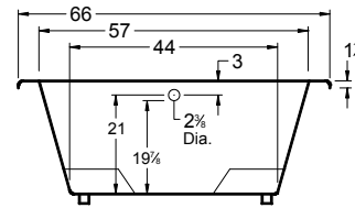
All bathtub dimensions are ± 1/2".
